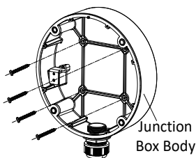
Figure 2-22 Secure the Junction Box's Body on Wall/Ceiling
