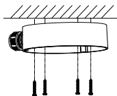
Figure 2-12 Fix the Junction Box
