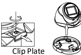
Figure 2-16 Remove the Clip Plate
