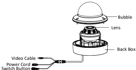
Figure 1-4 Type II Camera
