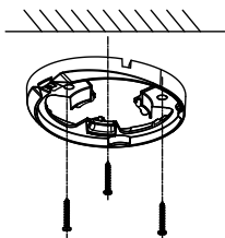
Figure 2-17 Install the Mounting Base to the Ceiling
