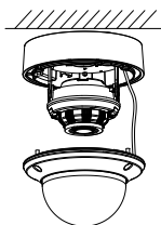
Figure 2-10 Install the Bubble Back
