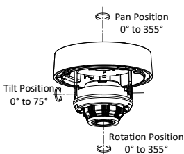
Figure 2-9 3-Axis Adjustment
