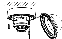
Figure 2-8 Attach the Back Box
