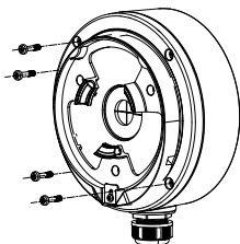
Figure 2-23 Fix the Junction Box
