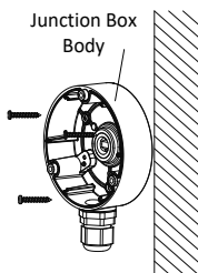
Figure 2-4 Secure the Junction Box on the Wall/Ceiling
